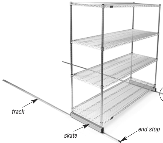
single deep unit shown assembled with wire starter unit
