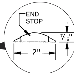
dimensions of floor track
