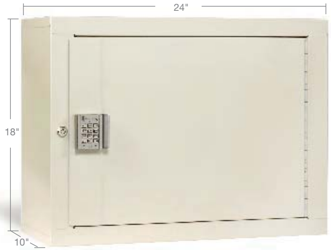
MHS-200 Medium High-Security Cabinet One Height Adjustable Tray Shelf w/2 dividers One Fixed Shelf Audit Trail Ready Shipping Weight 68lbs
