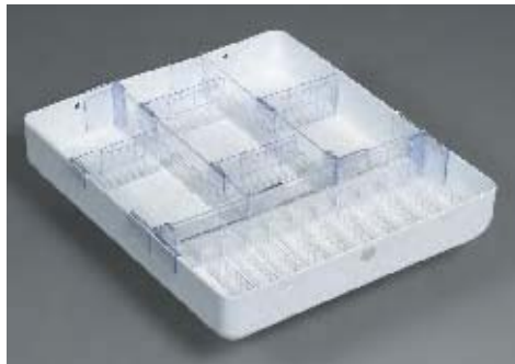
TMH-10 Mini Cart Tray with 4 dividers and 10 ampule holders, 2 rails 14"W x 16"D x 2½/16"H
