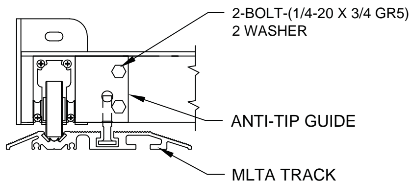
Detail of Anti-Tip Guide
